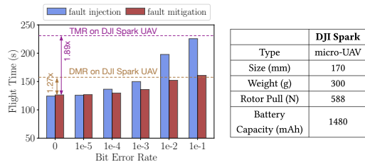
Figure 6: Comparison of software-based lightweight fault detection and recovery scheme [54] and redundancy-based approaches (DMR and TMR) on DJI Spark UAV platform from end-to-end autonomous system flight performance perspective.
